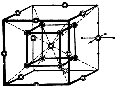
FIG. 2.—The K 2 [PtCl 6 ] structure. The black-centered circles represent the K + ions and the white-centered circles represent the Pt of the [PtCl 6 ] 2- ions. The whole complex ion is shown only in the case of the Pt at the extreme right where the six chlorines are shown as small solid circles.
